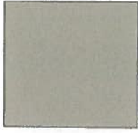
Clay PHS4-C0029
