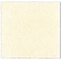
Almond PHS4-C0026
